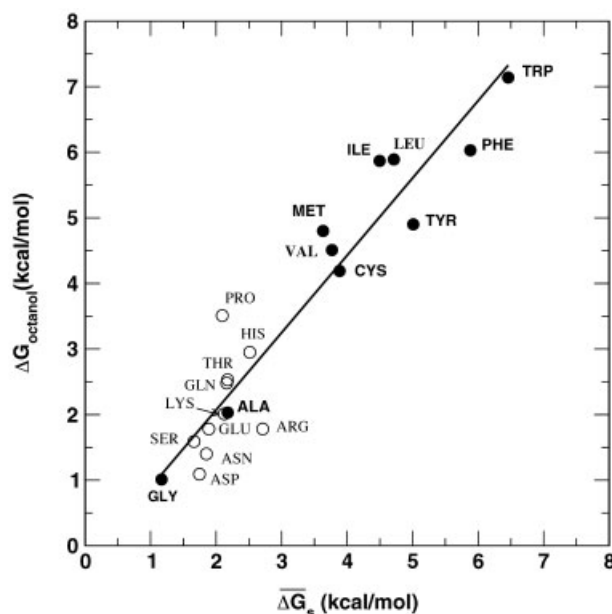
Fig. 1. The correlation between the corrected octanol to water transfer free energy and \overline{\Delta G}_s . The line is regression line for all residues. There is no significant correlation for hydrophilic residues ( R = 0.51 , open circles).
